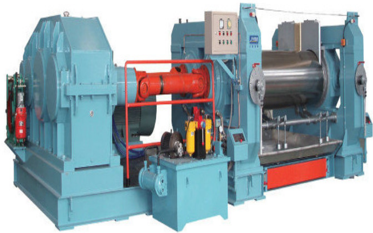
Machine: Mixing Mill with Chilled Cast Iron Cylinder
